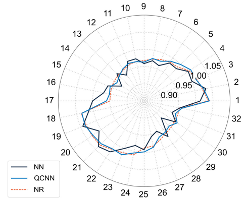
Fig. 13. Comparison of \vec{v} obtained from the NR and \vec{v} obtained from the NN and QCNN for the 33-bus test system under extreme conditions.
