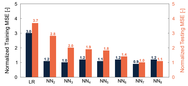
Fig. 8. Illustration of the impact of the NN architecture depth on the training and testing MSE for the 4-bus test system. Linear regression (LR) serves as a benchmark model. NN architectures with varying numbers of hidden layers, ranging from two (NN 2 ) to eight (NN 8 ), are assessed. The MSE values are normalized relative to the testing MSE obtained for the NN 7 .
