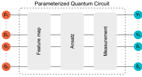
Fig. 4. Schematic depiction of the QNN designed for PF analysis, including a feature map, an ansatz, and the measurement. \vec{x} \in \{(\vec{p}_i, \vec{q}_i) : i = 1, 2, \dots, n\} and \vec{y} \in \{(\vec{v}_i, \vec{\delta}_i) : i = 1, 2, \dots, n\} respectively represent the input features and output labels, where n is the number of buses.
