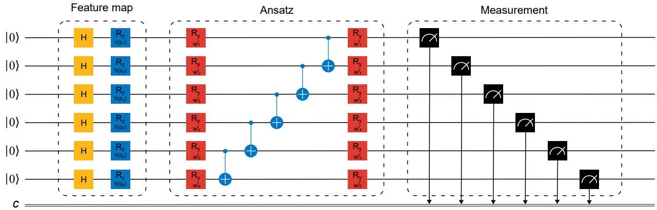
Fig. 9. Detailed representation of the PQC shown in Figure 4 for the 4-bus test system. \vec{x} \in \{(\vec{p}_i, \vec{q}_i) : i = 1, 2, \dots, n\} is initially encoded into a quantum state of multiple qubits using the feature map. Then, the data is processed through the ansatz. The feature map utilizes the Hadamard gate H and a rotation around the z-axis R_z on individual qubits. The ansatz applies a y-rotation R_y(\vec{w}_i^r) , followed by a CNOT gate, and subsequently another y-rotation R_y(\vec{w}_i^r) on each qubit. The expectation value for each qubit is then obtained within the interval of [-1, 1] from the measurement in the Z-basis.
