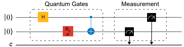
Fig. 3. Schematic representation of a PQC involving a pair of qubits. It includes both parameterized gate R_y(w^r) with adjustable parameter w^r , and non-parameterized gate H . CNOT gate entangles the second qubit to the first, executing a two-qubit operation. Finally, the measurement is performed to determine the expectation values of the involved qubits.
