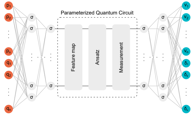
Fig. 5. Schematic depiction of the QCNN designed for PF analysis with a PQC replacing one hidden layer. \vec{x} \in \{(\vec{p}_i, \vec{q}_i) : i = 1, 2, \dots, n\} and \vec{y} \in \{(\vec{v}_i, \vec{\delta}_i) : i = 1, 2, \dots, n\} respectively represent the input features and output labels, where n is the number of buses. The data flow starts from a hidden layer, passes through the PQC, and continues to the subsequent hidden layer after the measurement.
